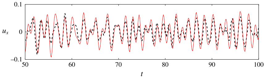
FIGURE 14. (Colour online) Comparison of the axial velocity computed from the TR-PIV snapshots (reference set, dashed line) and the reconstructed signal (red continuous line) at x=2.0 and r=0 (a point presenting an intermediate level of energy), for an arbitrary time range 50 < t < 100 .
