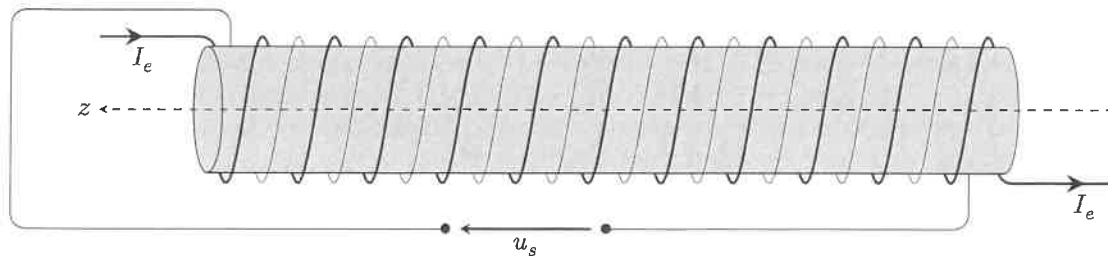
Figure 11 Fluxgate
